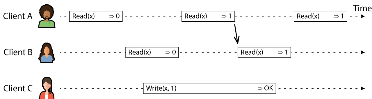
Figure 10-3. After any one read has returned the new value, all following reads (on the same or other clients) must also return the new value.
