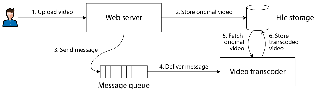
Figure 10-5. The web server and video transcoder communicate through both file storage and a message queue, opening the potential for race conditions.
