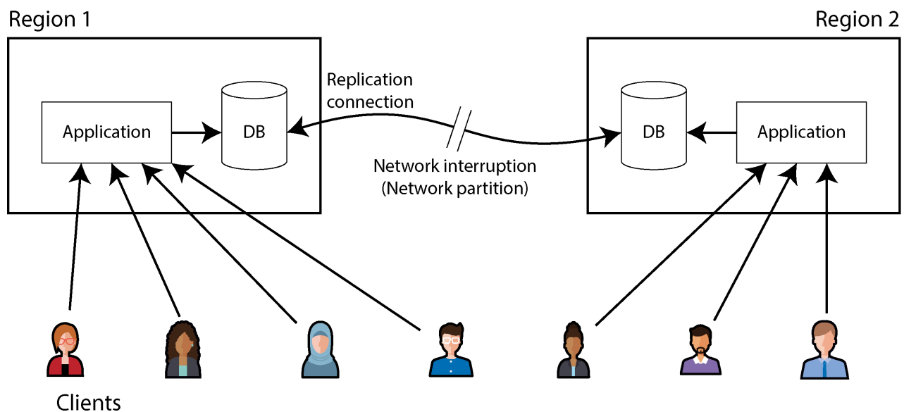
Figure 10-7. A network interruption forcing a choice between linearizability and availability
