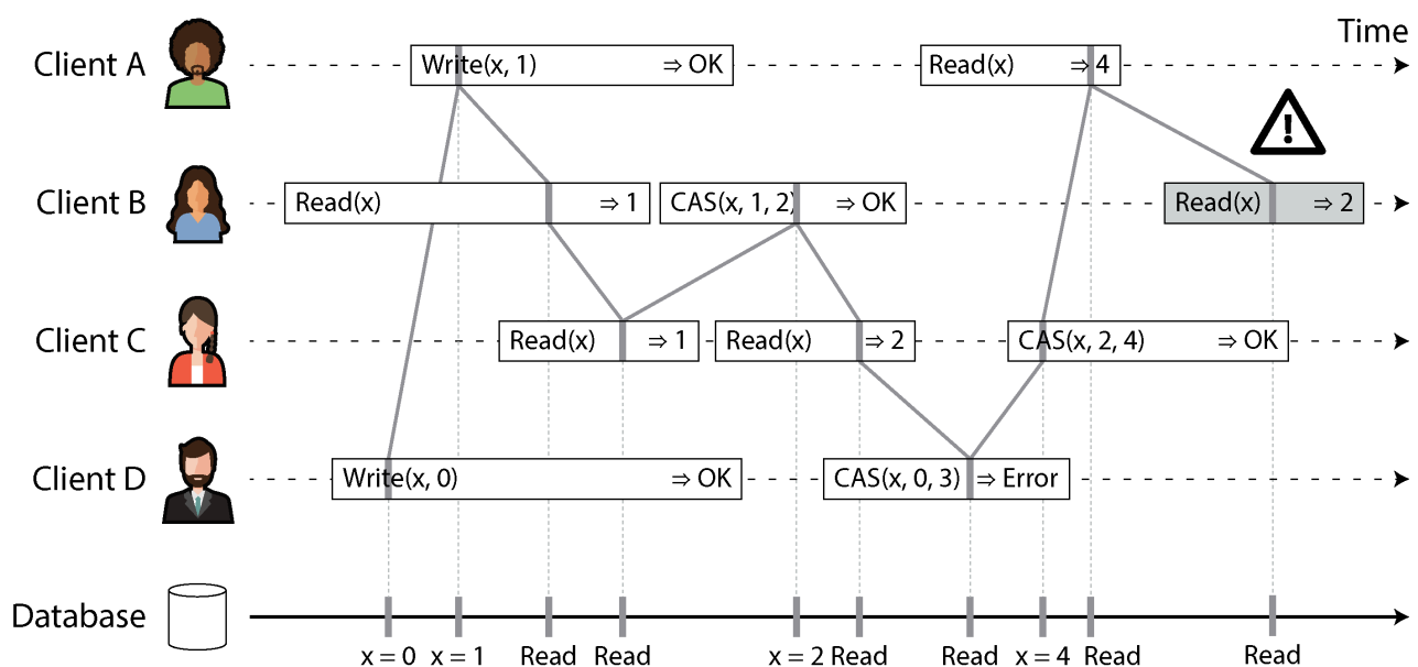
Figure 10-4. Visualizing the points in time at which the reads and writes appear to have taken effect—the final read by B is not linearizable
