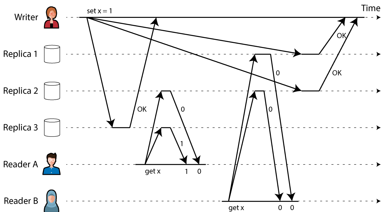
Figure 10-6. A nonlinearizable execution, despite using a quorum
